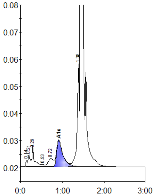
Peak table - ID: 10213181
