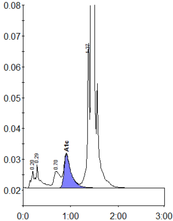
Peak table - ID: 10212636
