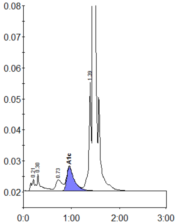
Peak table - ID: 10202541
