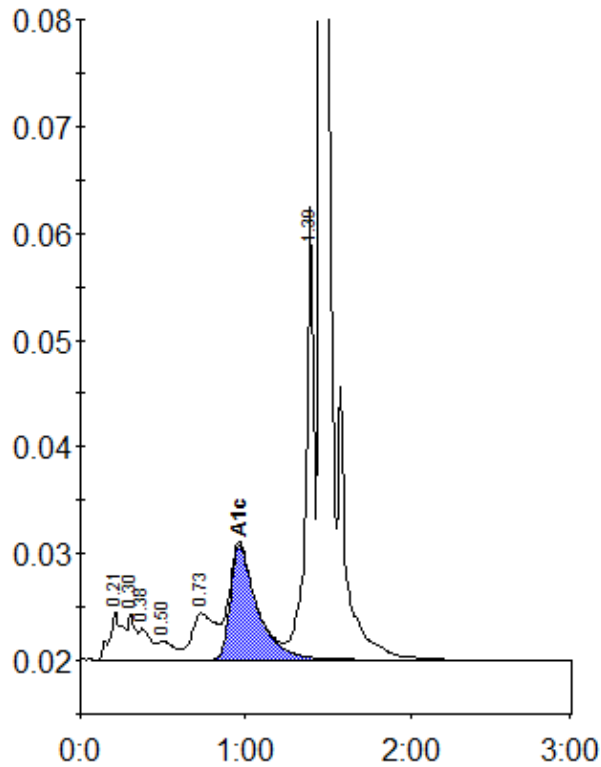
Peak table - ID: 10201129
