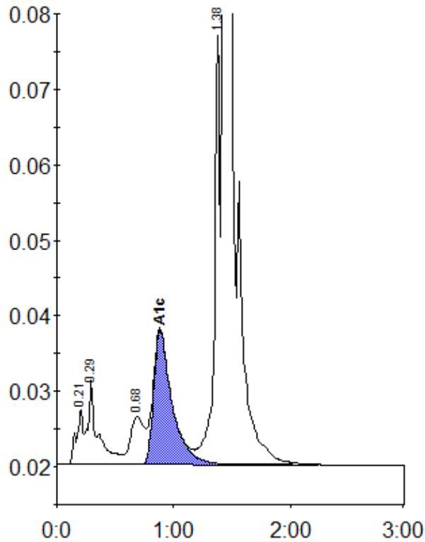
Peak table - ID: 10193407
