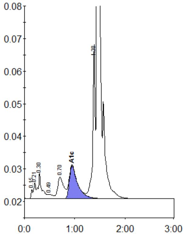
Peak table - ID: 10186032
