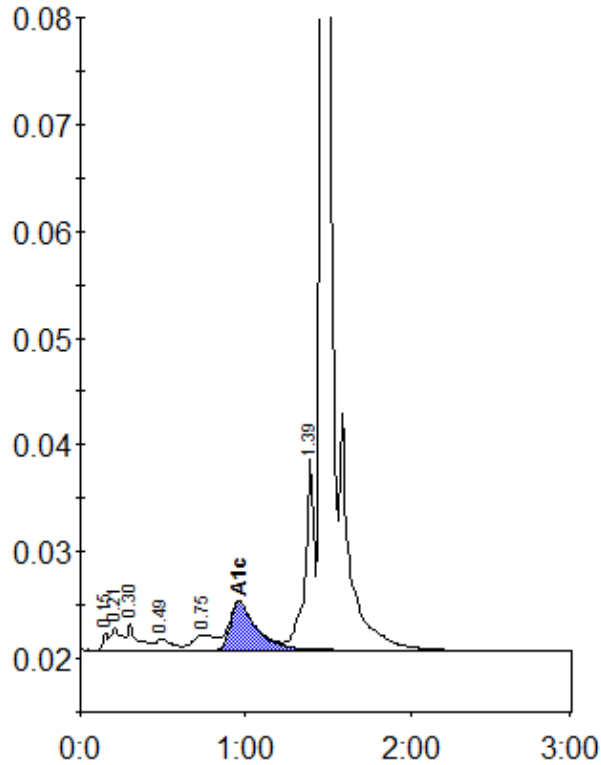
Peak table - ID: 10180098
