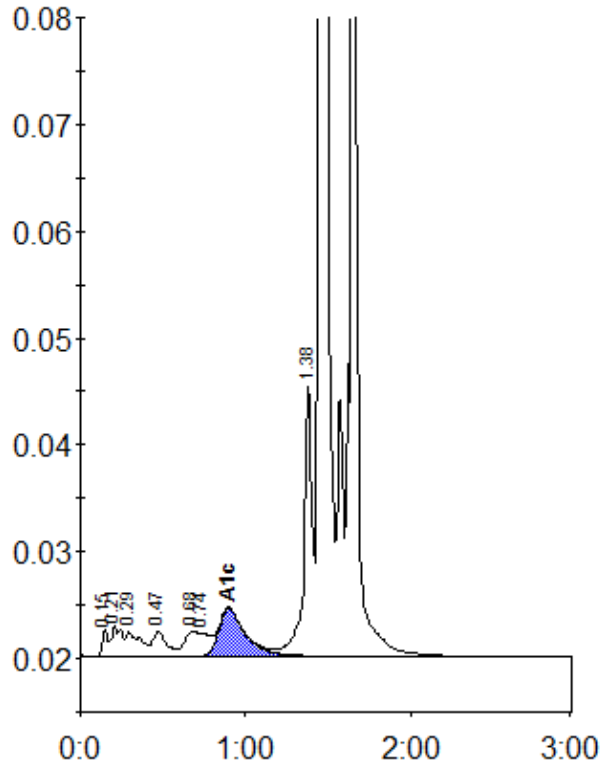
Peak table - ID: 10179554
