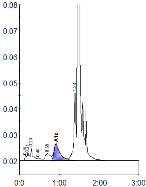
Peak table - ID: 10179154
