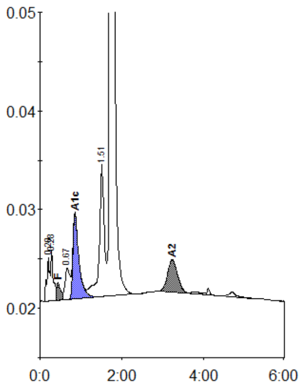
Peak table - ID: 10164603
