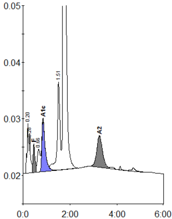
Peak table - ID: 10103697
