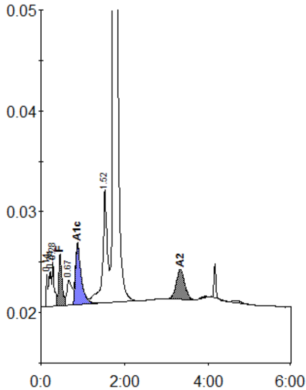
Peak table - ID: 10061125
